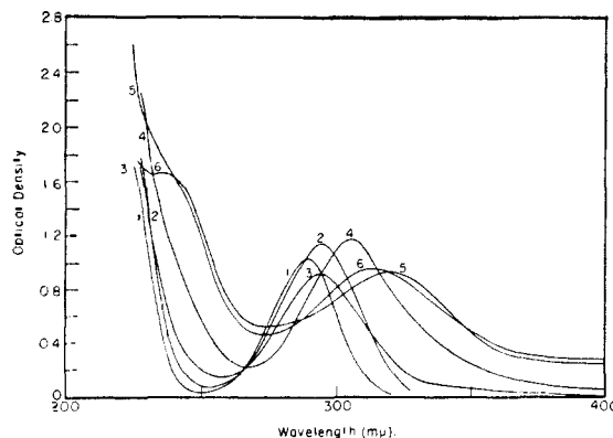
Fig. 8.—Change in ultraviolet absorption of the product of the quinhydrone–sulfite reaction with pH . 5.00 \times 10^{-3} M quinhydrone treated with 1.00 \times 10^{-2} M sulfite and product diluted 25-fold. The pH given is that of the diluted solution: curve 1, pH 1.66; curve 2, pH 6.72; curve 3, pH 8.50; curve 4, pH 9.12; curve 5, pH 10.08; curve 6, pH 10.66.
