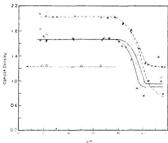
Fig. 6.—Change in optical density of three hydroquinones ( 4.00 \times 10^{-4} M ) with pH at maximum absorption: \circ \dots \circ , hydroquinone, D_{288.5} ; \oplus \dots \oplus , hydroquinone monosulfonate, D_{300.5} ; \circ \dots \circ , hydroquinone monosulfonate in presence of 4.00 \times 10^{-3} M sulfite, D_{300.5} ; \oplus \dots \oplus , hydroquinone disulfonate, D_{313} ; \circ \dots \circ , hydroquinone disulfonate in presence of 4.00 \times 10^{-3} M sulfite, D_{313} .
