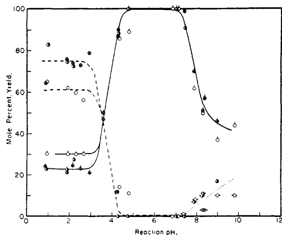
Fig. 10.—Variation of the mole per cent. yield of hydroquinone, hydroquinone monosulfonate and hydroquinone disulfonate with pH for the reaction of sulfite and quinone. Hydroquinone: \oplus , sulfite-quinone ratio = 1; \ominus , sulfite-quinone ratio = 2; \circ , sulfite-quinone ratio = 10. Hydroquinone monosulfonate: \oplus , sulfite-quinone ratio = 1; \ominus , sulfite-quinone ratio = 2; \circ , sulfite-quinone ratio = 10. Hydroquinone disulfonate: -\oplus- , sulfite-quinone ratio = 1; -\ominus- , sulfite-quinone ratio = 2; -\circ- , sulfite-quinone ratio = 10.
