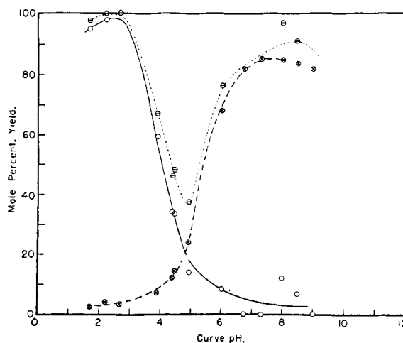
Fig. 12.—Variation of the mole per cent. yield of hydroquinone monosulfonate and hydroquinone disulfonate with pH for the reaction of sulfite and quinone monosulfonate. The sulfite-quinone monosulfonate ratio is 10. \circ , hydroquinone monosulfonate; \oplus , hydroquinone disulfonate; \ominus , total accountable product.
