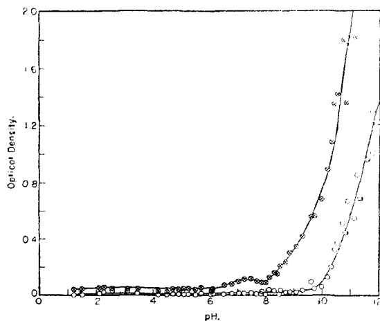
Fig. 2.—Variation in optical density of the sulfite-quinone reaction product, at 400 and 610 m\mu , with pH : \circ , D_{610} ; \otimes , D_{400} .
