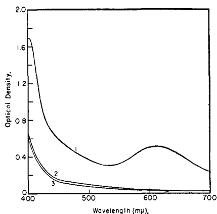
Fig. 4.—Greenish-blue intermediate in pH 12.2 phosphate buffer: curve 1, quinone and large excess of sulfite; curve 2, Eastman Kodak quinhydrone and large excess of sulfite; curve 3, freshly prepared quinhydrone and large excess of sulfite. The quinhydrone does not yield a greenish-blue intermediate.
