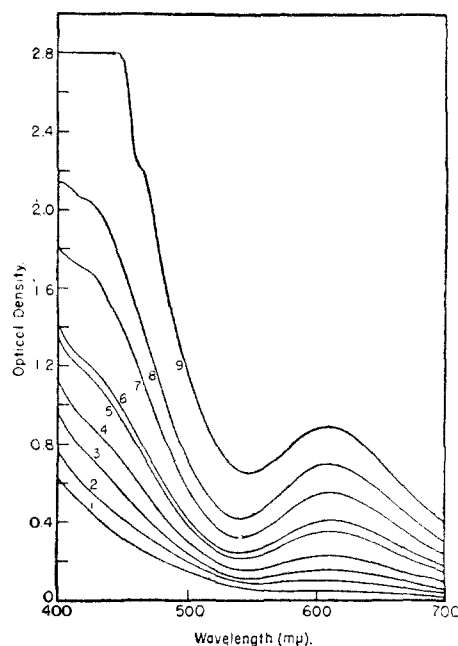
Fig. 1.—Density curves for the greenish-blue intermediate at several values of pH in carbonate buffer. Sulfite-quinone ratio is unity; curve 1, pH 9.72; curve 2, pH 9.99; curve 3, pH 10.18; curve 4, pH 10.32; curve 5, pH 10.43; curve 6, pH 10.54; curve 7, pH 10.72; curve 8, pH 10.90; curve 9, pH 11.20.
