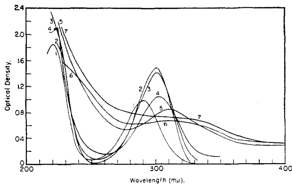
Fig. 7.—Change in ultraviolet absorption of the product of the quinone–sulfite reaction with pH . 1.00 \times 10^{-2} M quinone treated with 1.00 \times 10^{-2} M sulfite and product diluted 25-fold. The pH given is that of the diluted solution: curve 1, pH 2.04; curve 2, pH 4.38; curve 3, pH 7.14; curve 4, pH 8.42; curve 5, pH 9.62; curve 6, pH 10.18; curve 7, pH 11.05.
