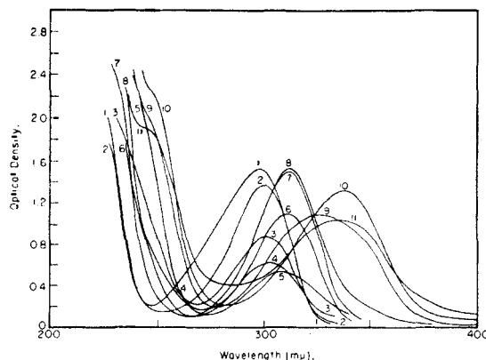
Fig. 9.—Change in ultraviolet absorption of the product of the quinone–monosulfonate–sulfite reaction, with pH . 3.6 \times 10^{-4} M quinone monosulfonate treated with 3.60 \times 10^{-3} M sulfite: curve 1, pH 1.67; curve 2, pH 3.90; curve 3, pH 4.40; curve 4, pH 4.96; curve 5, pH 6.02; curve 6, pH 7.30; curve 7, pH 8.50; curve 8, pH 9.71; curve 9, pH 10.64; curve 10, pH 11.66.
