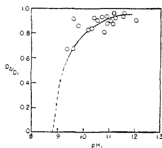
Fig. 3.—Variation in stability of the greenish-blue intermediate with pH .
