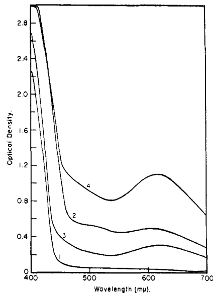
Fig. 5.—Intermediates resulting from reaction of sulfhydryl compounds and quinone in pH 12.2 phosphate buffer: curve 1, 5-fold excess of cysteine; curve 2, 1:1 compound of cysteine and sulfite; curve 3, 5-fold excess of glutathione; curve 4, 1:1 compound of glutathione and quinone.
