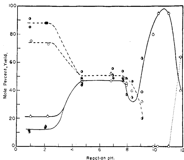
Fig. 11.—Variation of the mole per cent. yield of hydroquinone, hydroquinone monosulfonate, and hydroquinone disulfonate with pH for the reaction of sulfite and quinhydrone. Hydroquinone: \oplus , sulfite-quinone ratio = 2; \ominus , sulfite-quinone ratio = 4; \circ , sulfite-quinone ratio = 20. Hydroquinone monosulfonate: \oplus , sulfite-quinone ratio = 2; \ominus , sulfite-quinone ratio = 4; \circ , sulfite-quinone ratio = 20. Hydroquinone disulfonate: -\oplus- , sulfite-quinone ratio = 2; -\ominus- , sulfite-quinone ratio = 4; -\circ- , sulfite-quinone ratio = 20.
